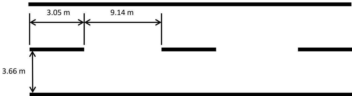
Figure 1 Lane Markings
