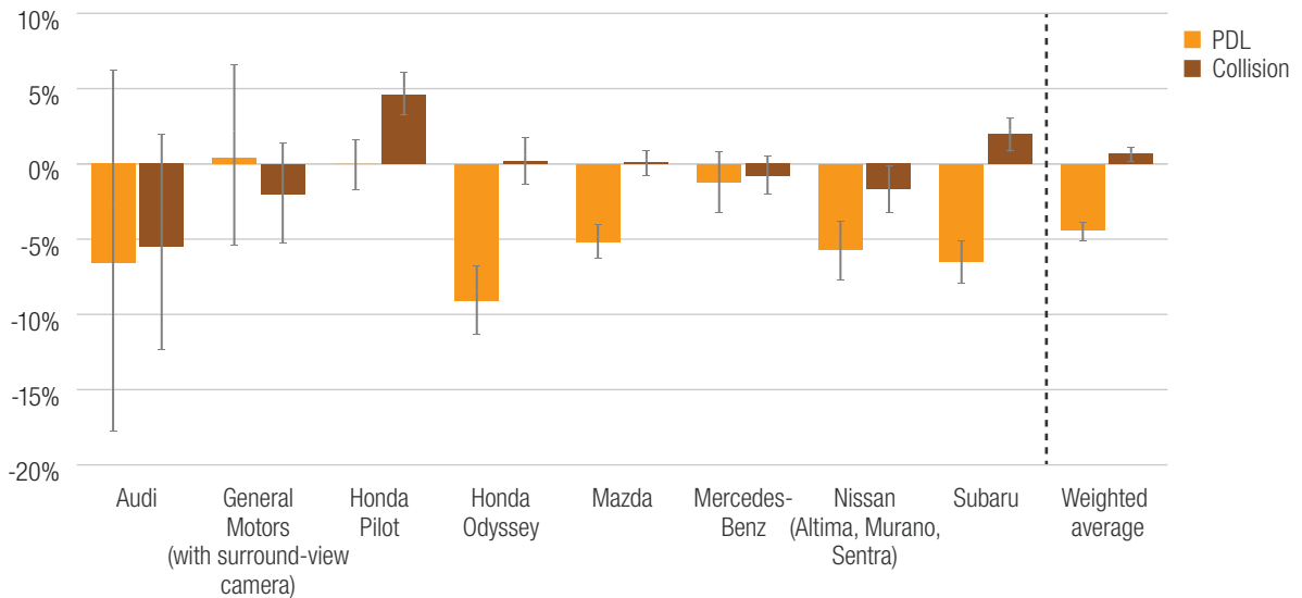
Figure 19: Change in PDL and collision claim frequency associated with rear cameras
