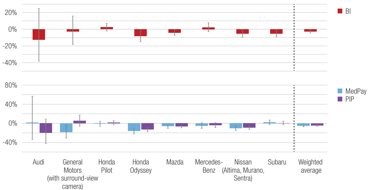
Figure 20: Change in BI liability, MedPay, and PIP claim frequency associated with rear cameras
