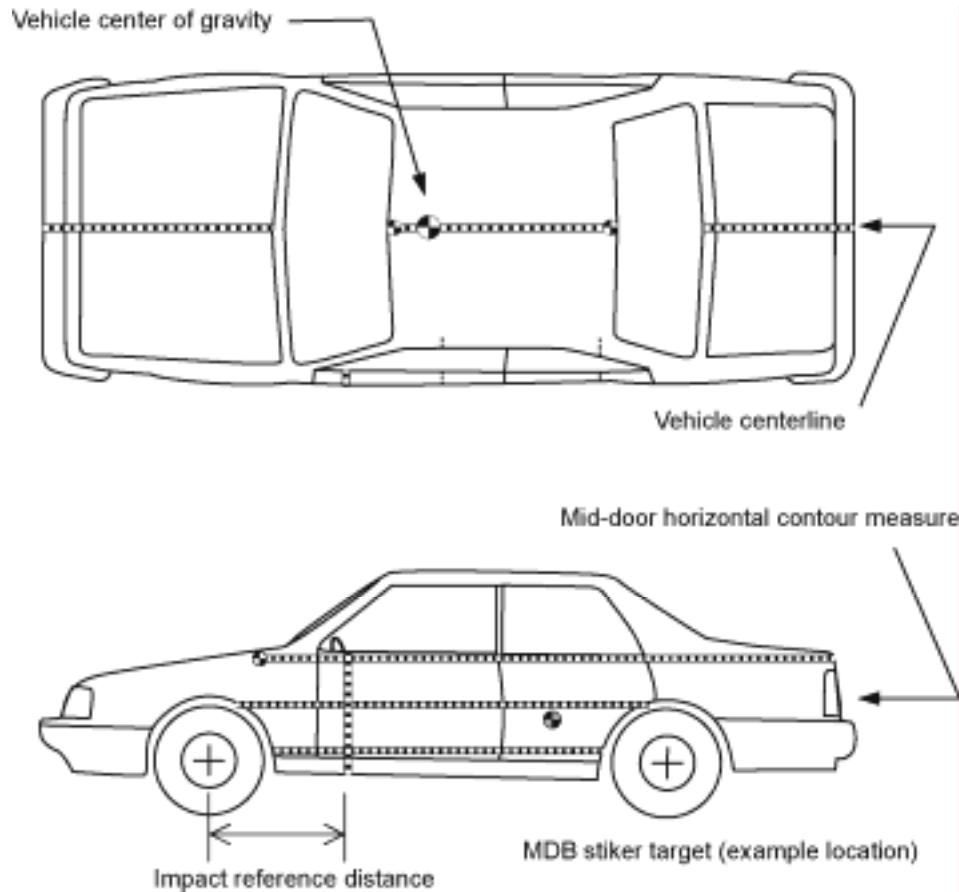
Figure 4 Exterior Surface Marking
