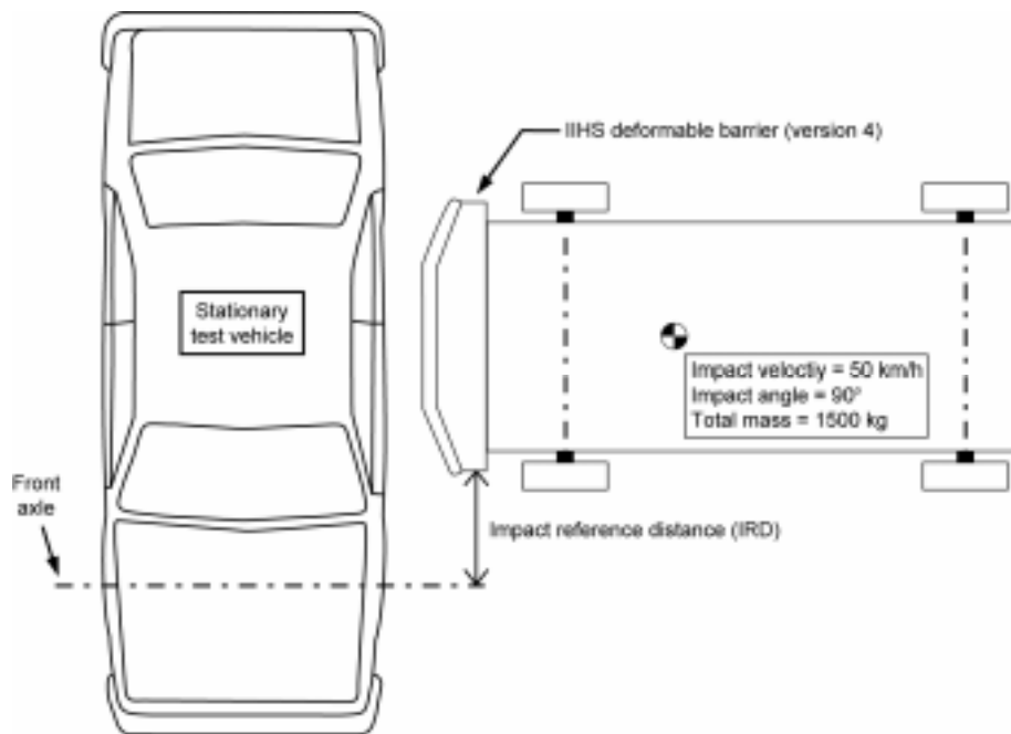
Figure 1 Moving Deformable Barrier Alignment with Test Vehicle
