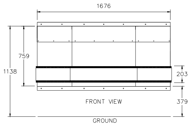
Figure 3 IIHS Deformable Barrier Element (Version 4) (all measurements in millimeters)
