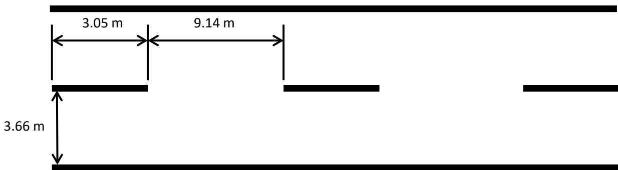
Lane markings
