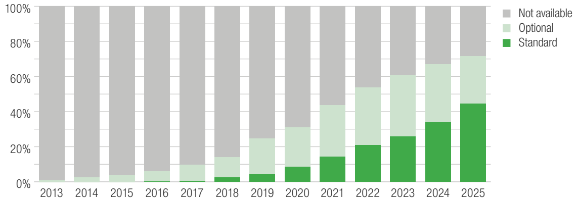
Figure 32: Percentage of new vehicle series with rear automatic emergency braking by model year
