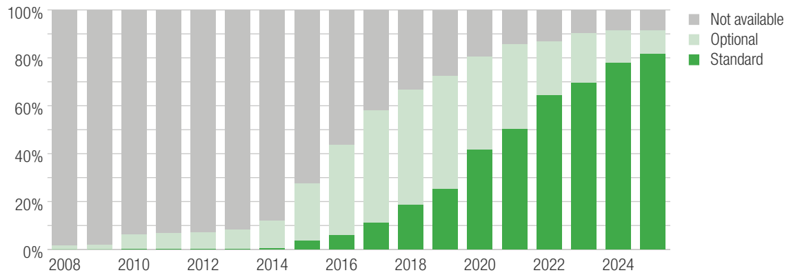
Figure 23: Percentage of new vehicle series with high-beam assist by model year
