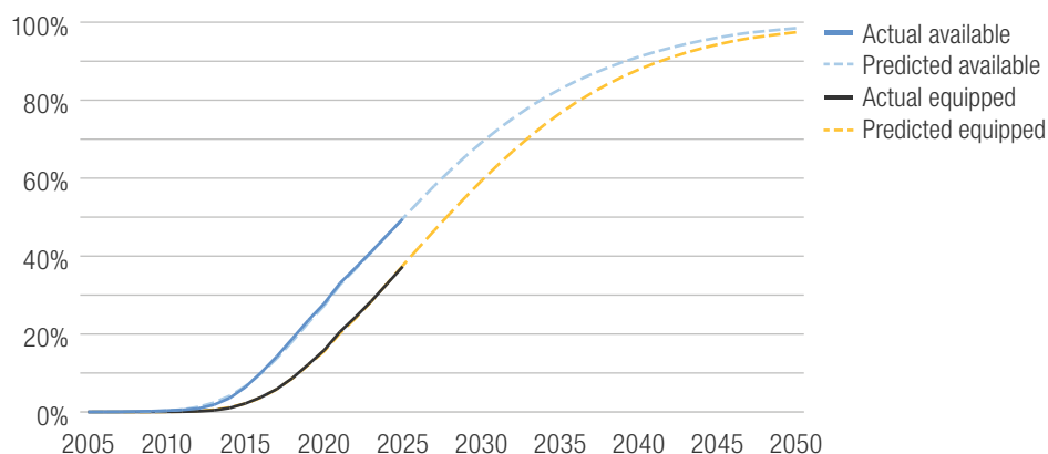
Figure 16: Predicted percentage of registered vehicles with lane departure warning by calendar year
