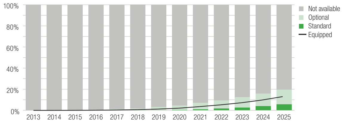
Figure 33: Percentage of registered vehicles with rear automatic emergency braking by calendar year
