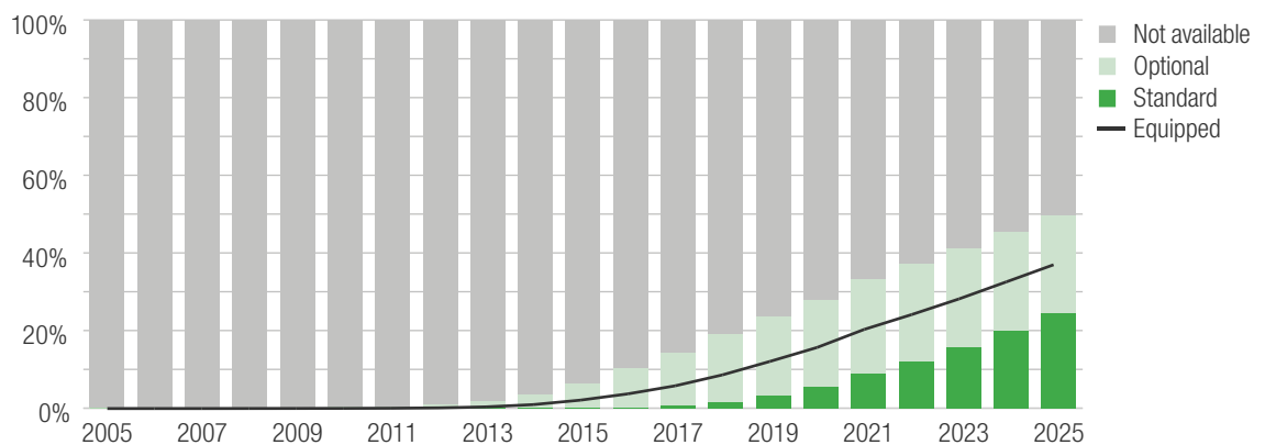
Figure 15: Percentage of registered vehicles with lane departure warning by calendar year
