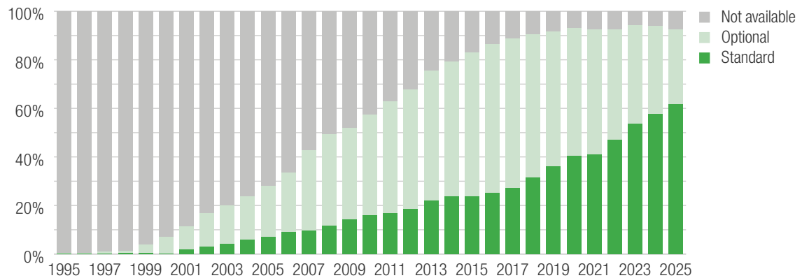
Figure 26: Percentage of new vehicle series with rear parking sensors by model year
