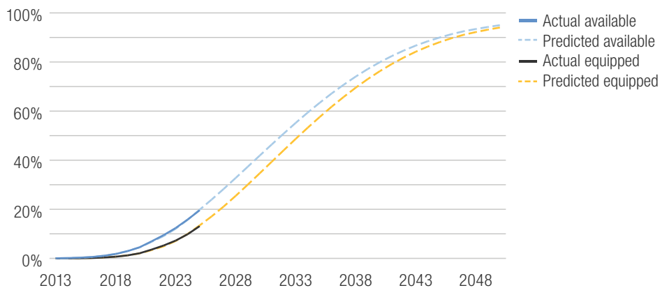
Figure 34: Predicted percentage of registered vehicles with rear automatic emergency braking by calendar year
