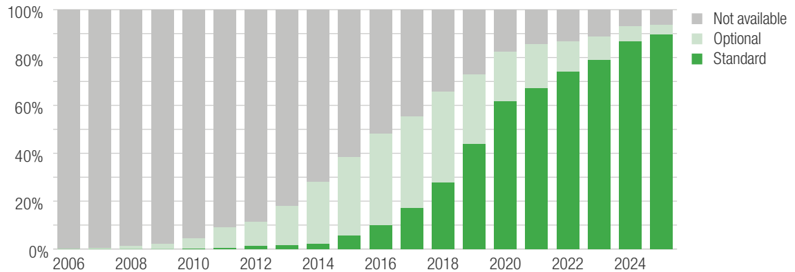
Figure 5: Percentage of new vehicle series with front automatic emergency braking by model year
