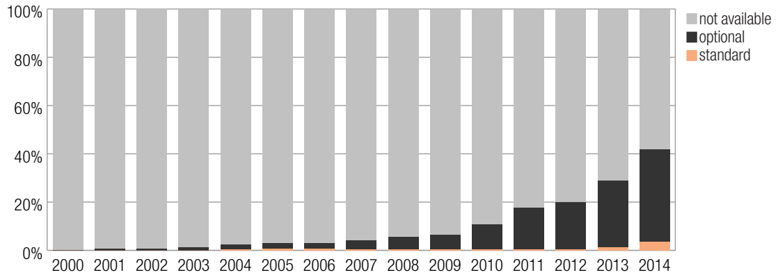
Figure 7: Percentage of new vehicle series with front crash prevention
