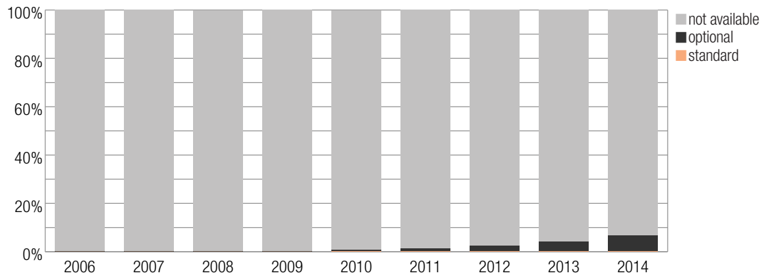
Figure 20: Percentage of registered vehicles with blind spot monitor
