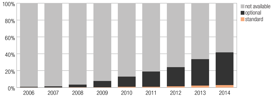
Figure 19: Percentage of new vehicle series with blind spot monitor
