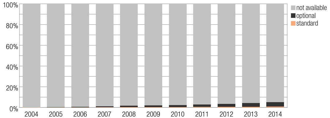
Figure 14: Percentage of registered vehicles with adaptive headlights
