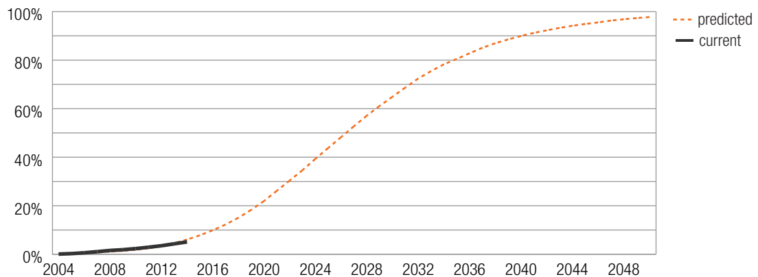
Figure 15: Predicted percentage of registered vehicles with available adaptive headlights
