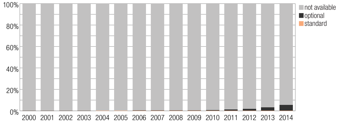
Figure 8: Percentage of registered vehicles with front crash prevention
