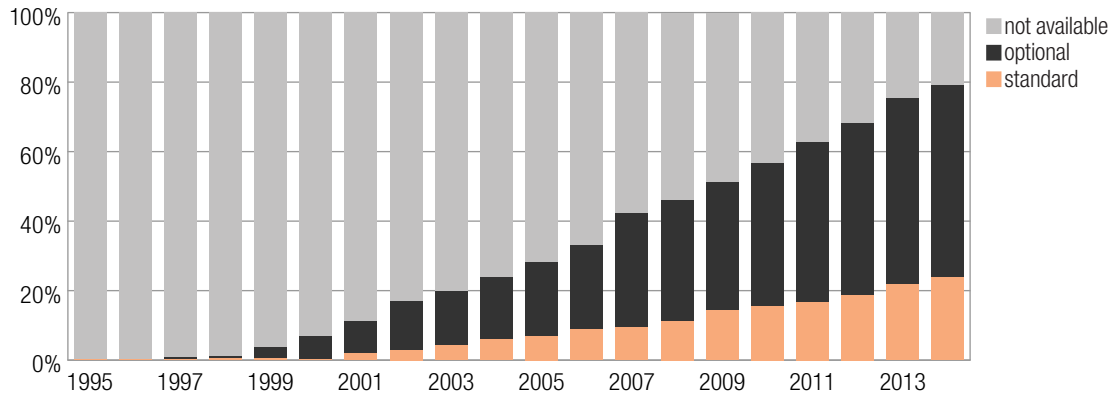
Figure 4: Percentage of new vehicle series with rear parking sensors
