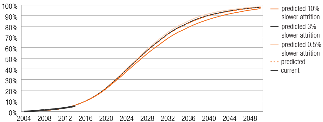
Appendix Figure 3: Predicted percentage of registered vehicles with adaptive headlights
