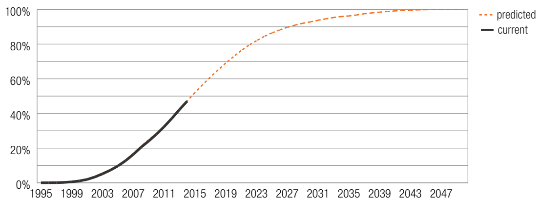
Figure 3: Predicted percentage of registered vehicles with available ESC
