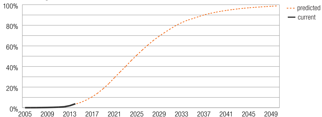
Figure 18: Predicted percentage of registered vehicles with available lane departure warning
