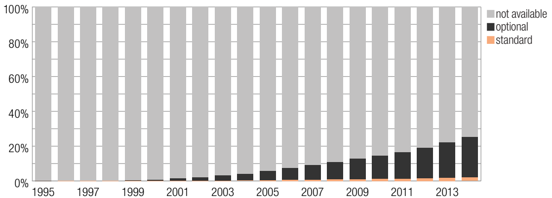
Figure 5: Percentage of registered vehicles with rear parking sensors
