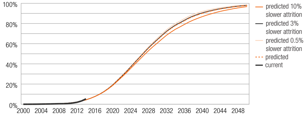
Appendix Figure 1: Predicted percentage of registered vehicles with front crash prevention
