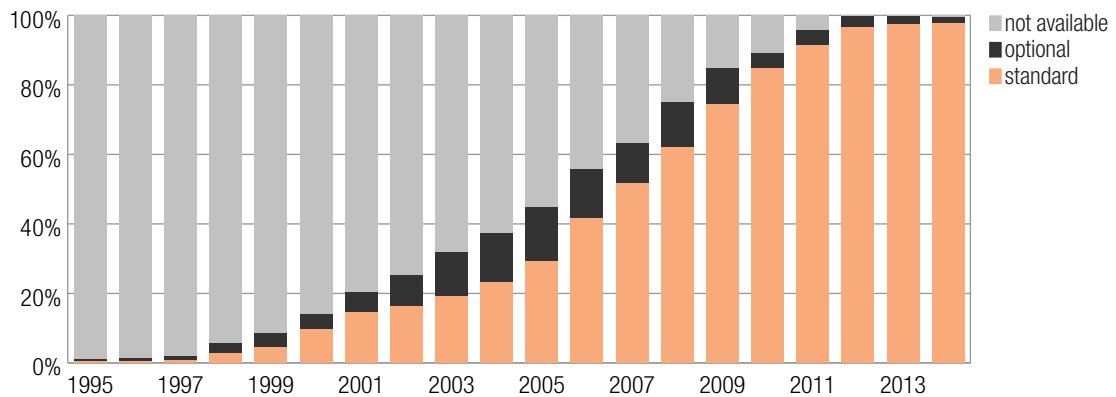
Figure 1: Percentage of new vehicle series with ESC
