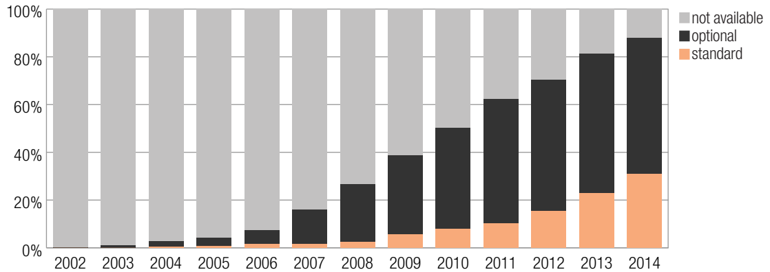
Figure 10: Percentage of new vehicle series with rear camera
