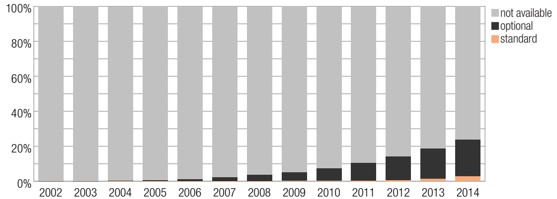
Figure 11: Percentage of registered vehicles with rear camera
