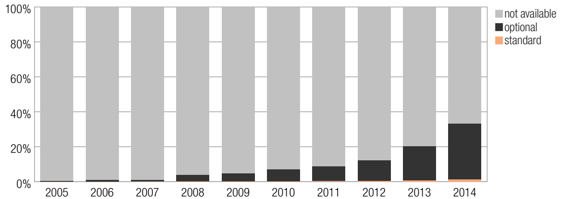
Figure 16: Percentage of new vehicle series with lane departure warning
