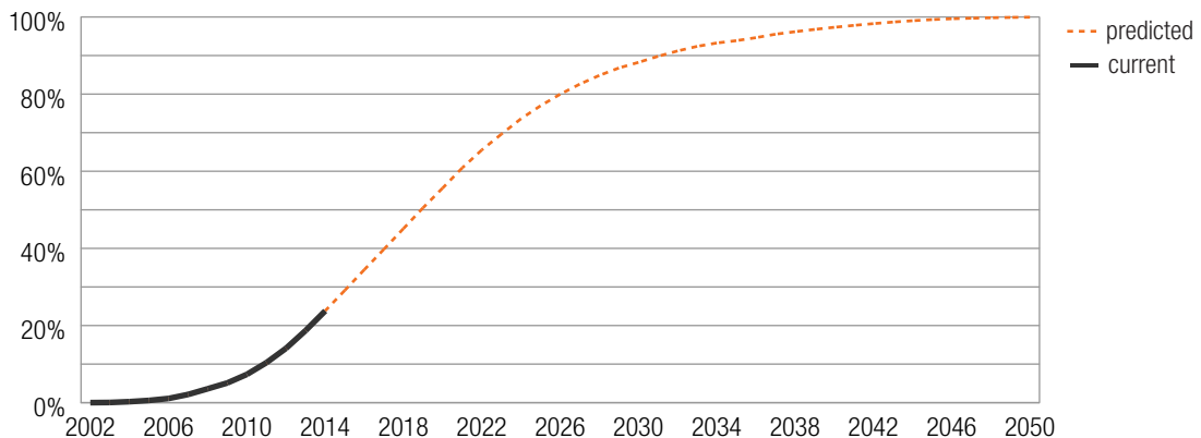
Figure 12: Predicted percentage of registered vehicles with available rear camera
