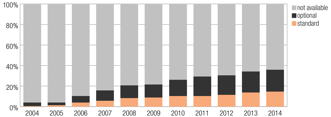
Figure 13: Percentage of new vehicle series with adaptive headlights
