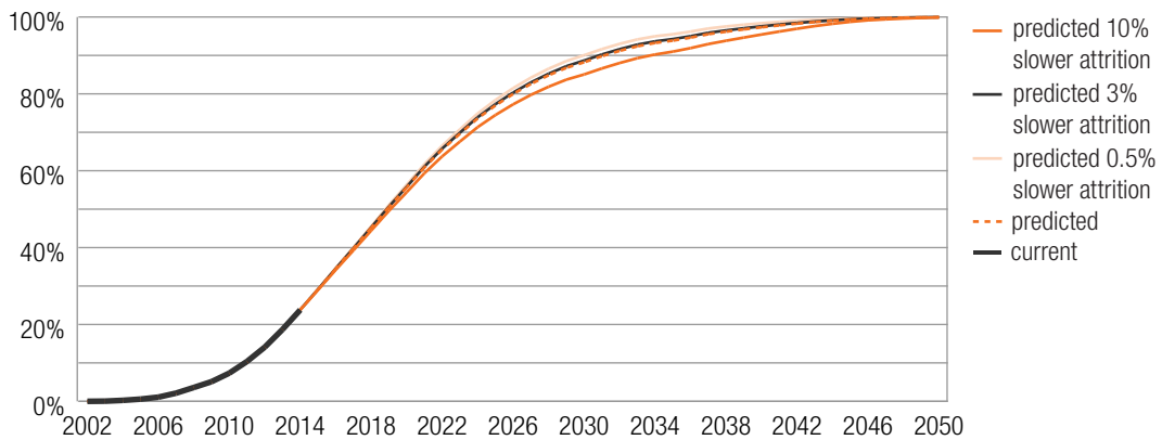
Appendix Figure 2: Predicted percentage of registered vehicles with rear camera
