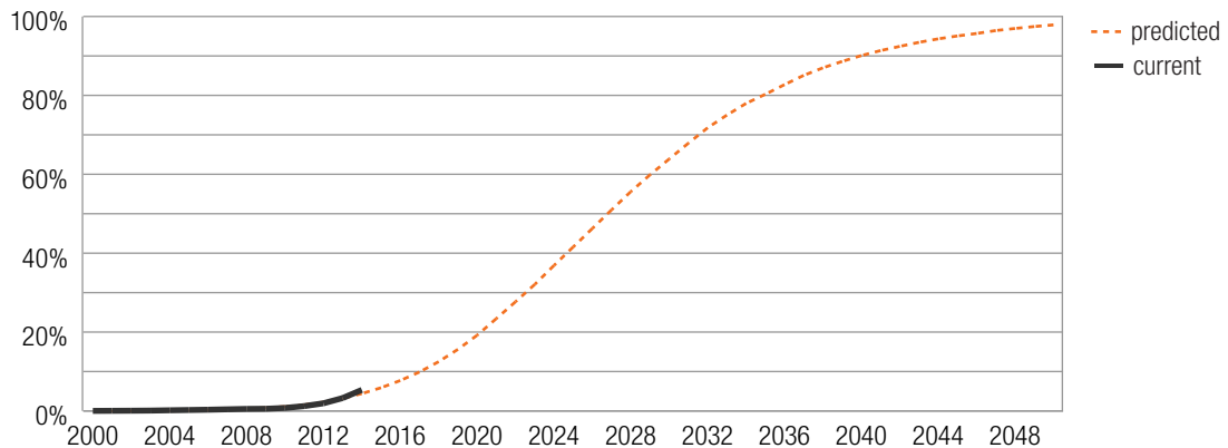
Figure 9: Predicted percentage of registered vehicles with available front crash prevention
