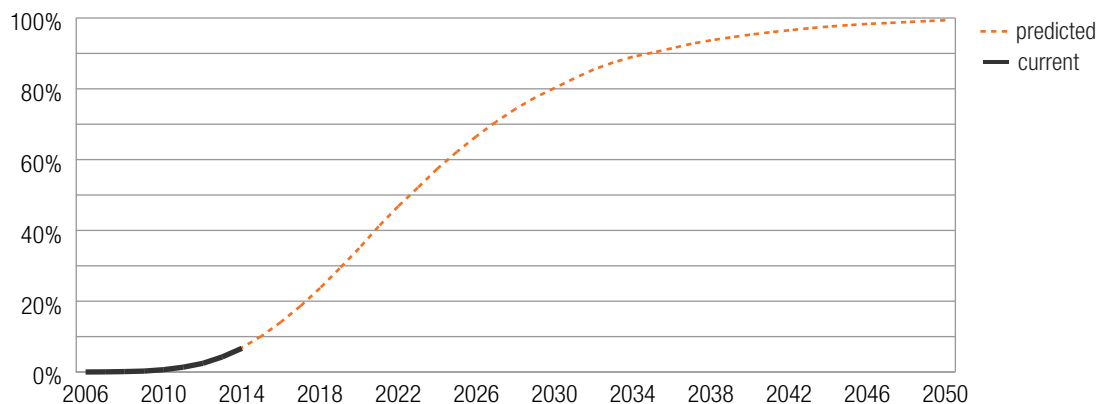
Figure 21: Predicted percentage of registered vehicles with available blind spot monitor
