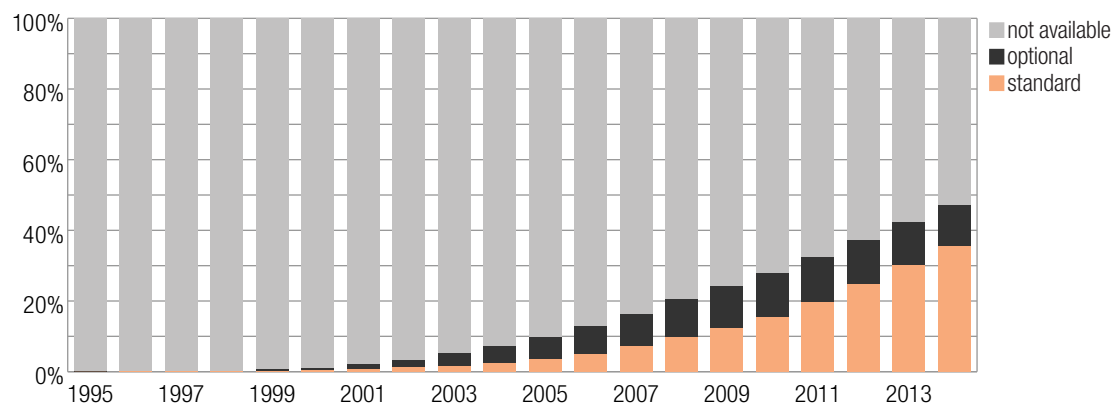
Figure 2: Percentage of registered vehicles with ESC
