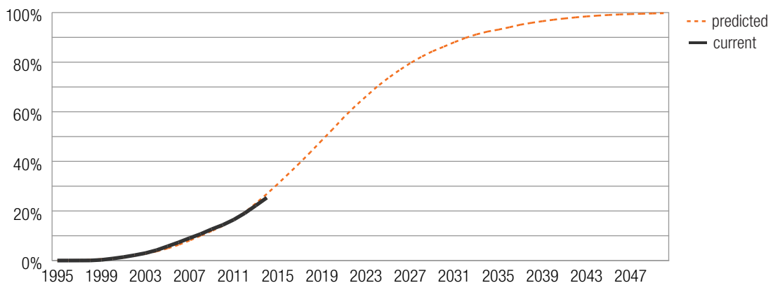
Figure 6: Predicted percentage of registered vehicles with available rear parking sensors
