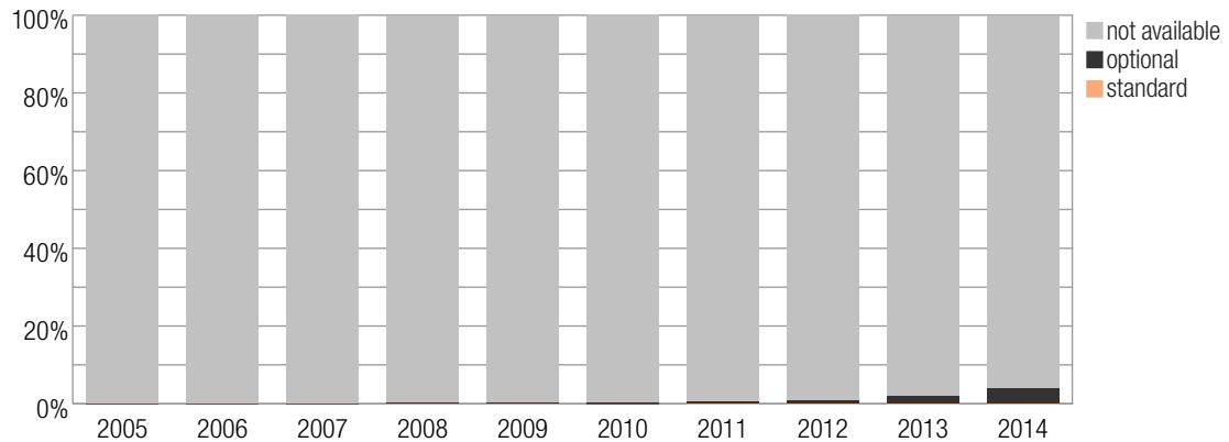
Figure 17: Percentage of registered vehicles with lane departure warning
