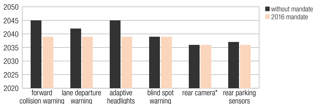
Calendar year features reach 95% of registered vehicle fleet with and without hypothetical mandate
