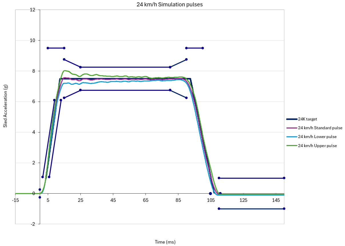
Figure C-4 24-km/h delta V crash pulses for simulation
