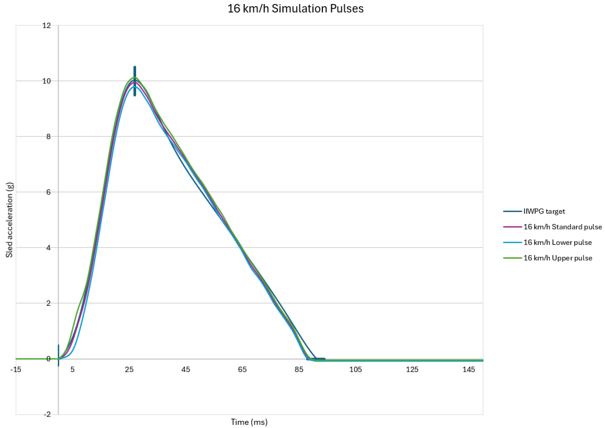
Figure C-3 16-km/h delta V crash pulses for simulation
