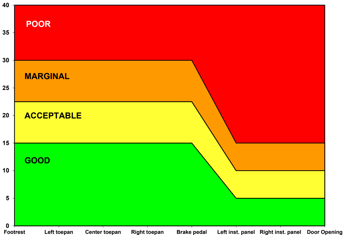
Figure 2 Guidelines for rating occupant compartment intrusion (cm)
