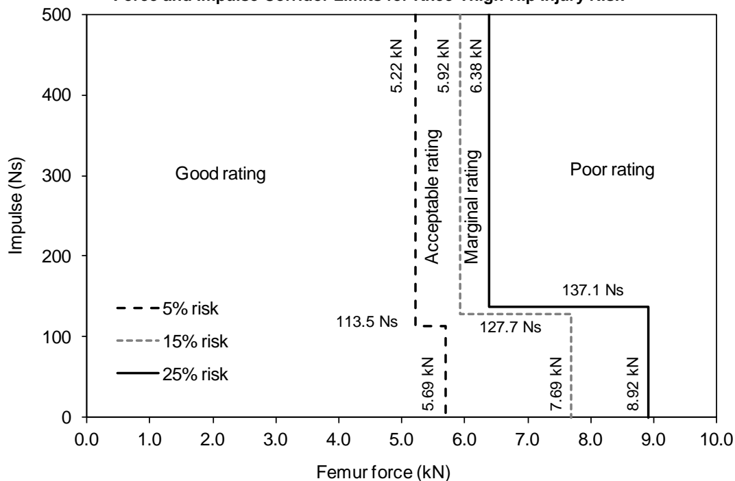
Figure 12 Force and Impulse Corridor Limits for Knee-Thigh-Hip Injury Risk
