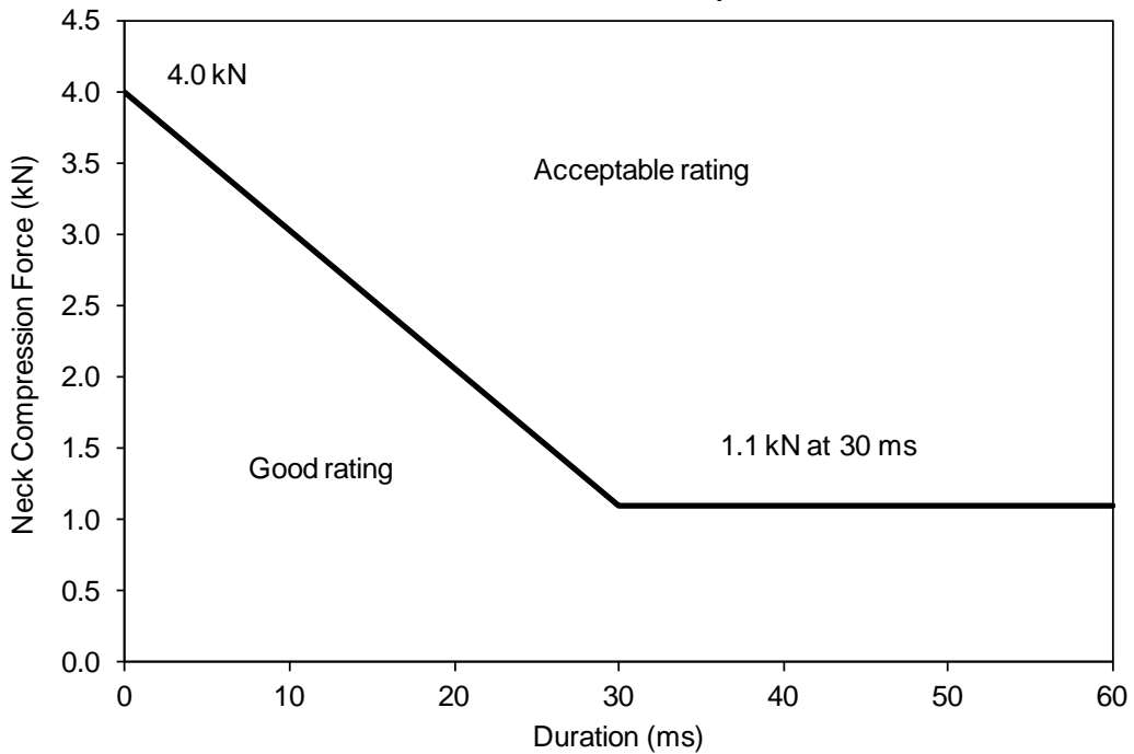
Figure 9 Force Duration Corridor for Neck Compression Force
