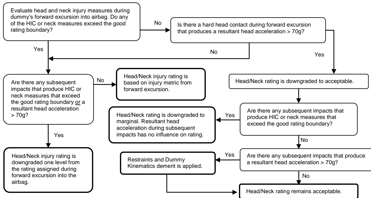
Figure 7 Flowchart: Influence of Multiple Impacts on Head/Neck Injury Rating
