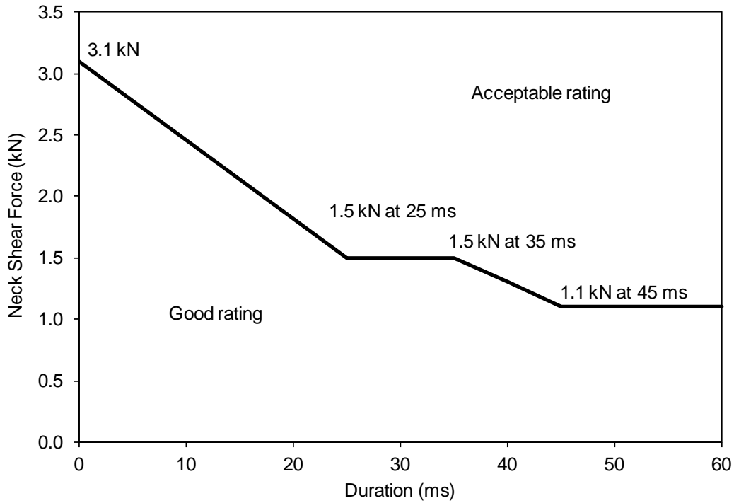
Figure 10 Force Duration Corridor for Neck Shear Force
