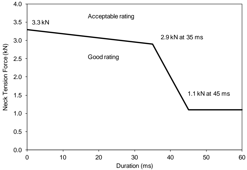
Figure 8 Force Duration Corridor for Neck Tension Force
