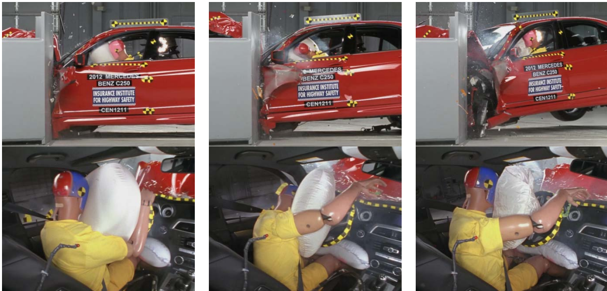
Figure 3 Example of Partial Frontal Airbag Interaction – 2012 Mercedes C250 (CEN1211)
