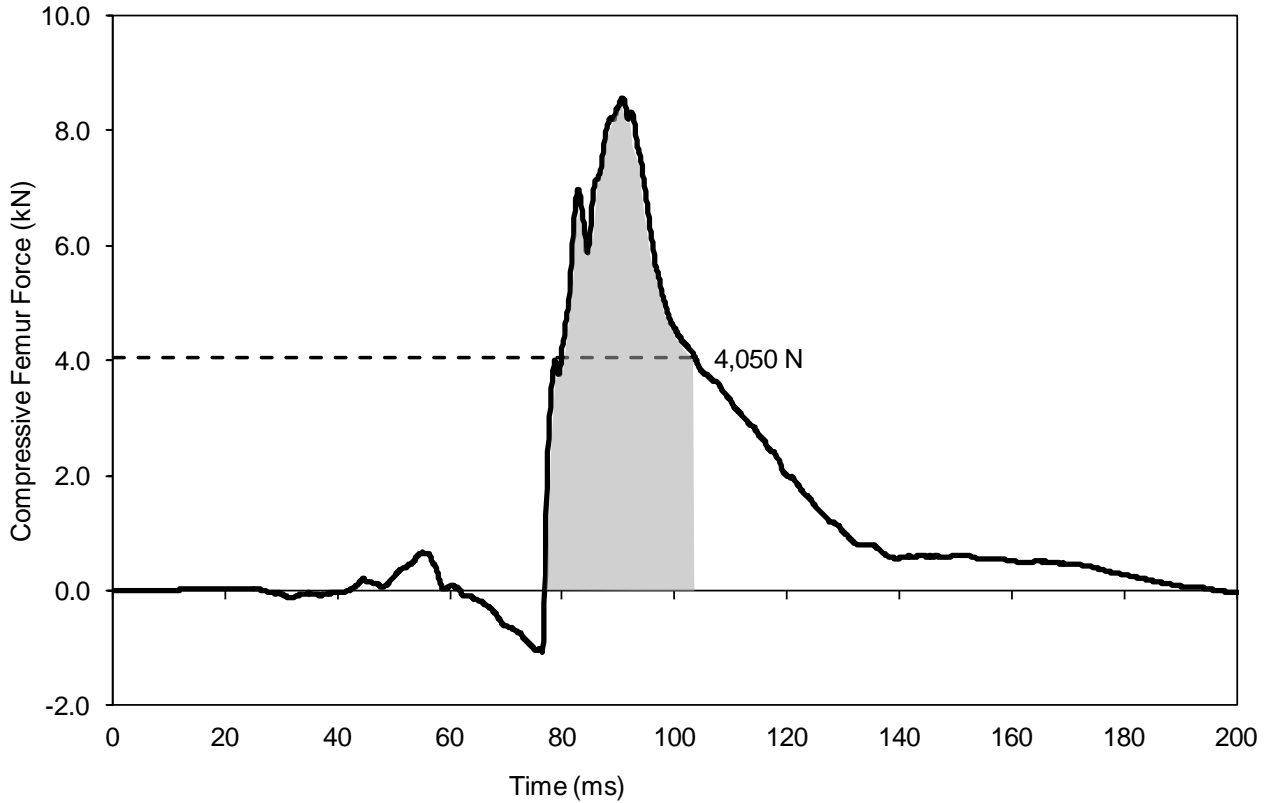
Figure 11 Integration Limits for Calculation of Femur Impulse for Hybrid III 50th Dummy
